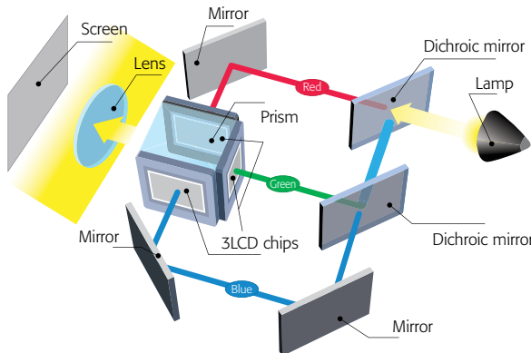
▲ 3LCD technology
